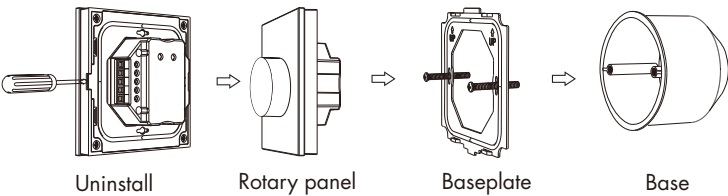
Installation diagram:
