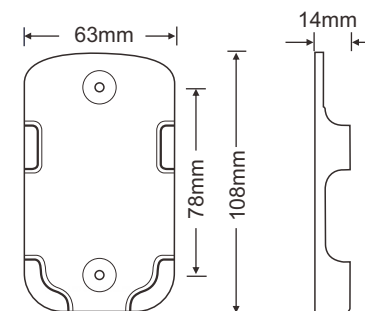
Remote holder
