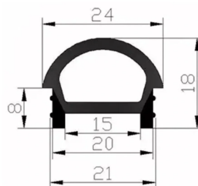
Cross-section — all dimensions in millimetres
