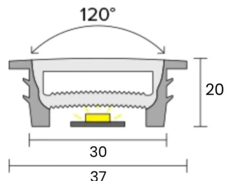
Cross-section — all dimensions in millimetres
