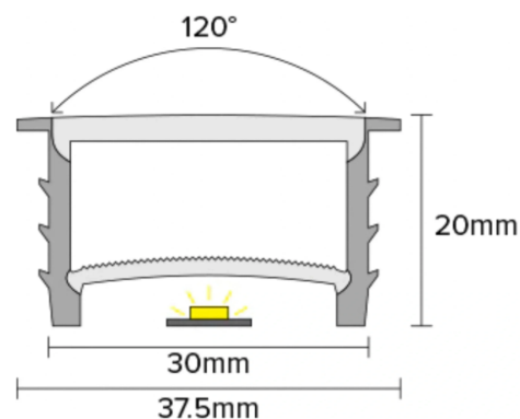
Cross-section — all dimensions in millimetres
