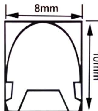
Cross-section — all dimensions in millimetres
