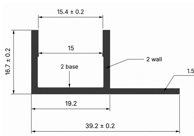
Cross-section in mm. Not to scale. Supplied drawing callouts; verify fit before installation.
