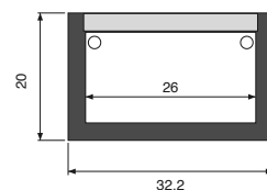
CN635 - Section 32.2 × 20mm - 26mm internal channel - fits neon flex up to 26mm
