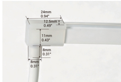
Bottom cable exit
