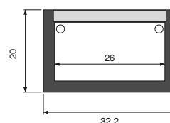
CN635 - Section 32.2 × 20mm - 26mm internal channel - fits neon flex up to 26mm
