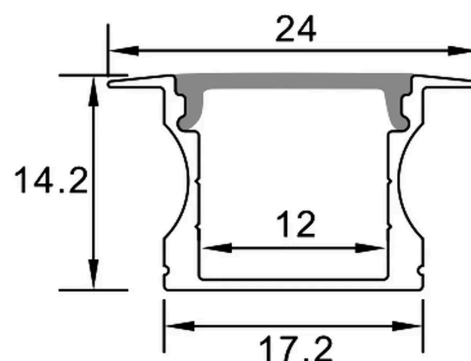
Cross-section — all dimensions in millimetres
