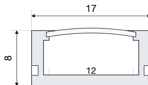
Cross-section — all dimensions in millimetres
