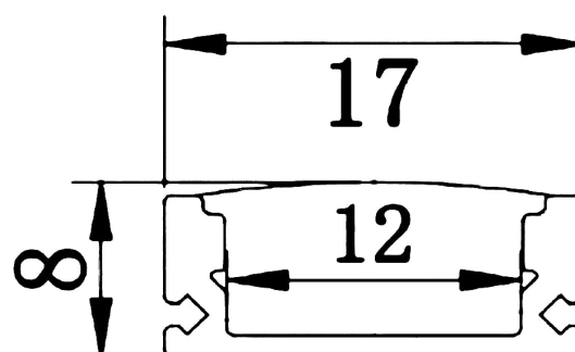
Cross-section — all dimensions in millimetres
