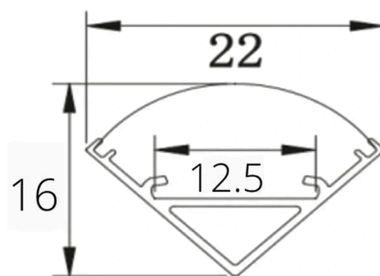
Cross-section — all dimensions in millimetres
