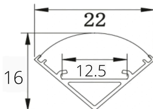
Cross-section — all dimensions in millimetres
